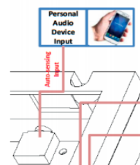
Input Jack for Mobile Phone Sound
